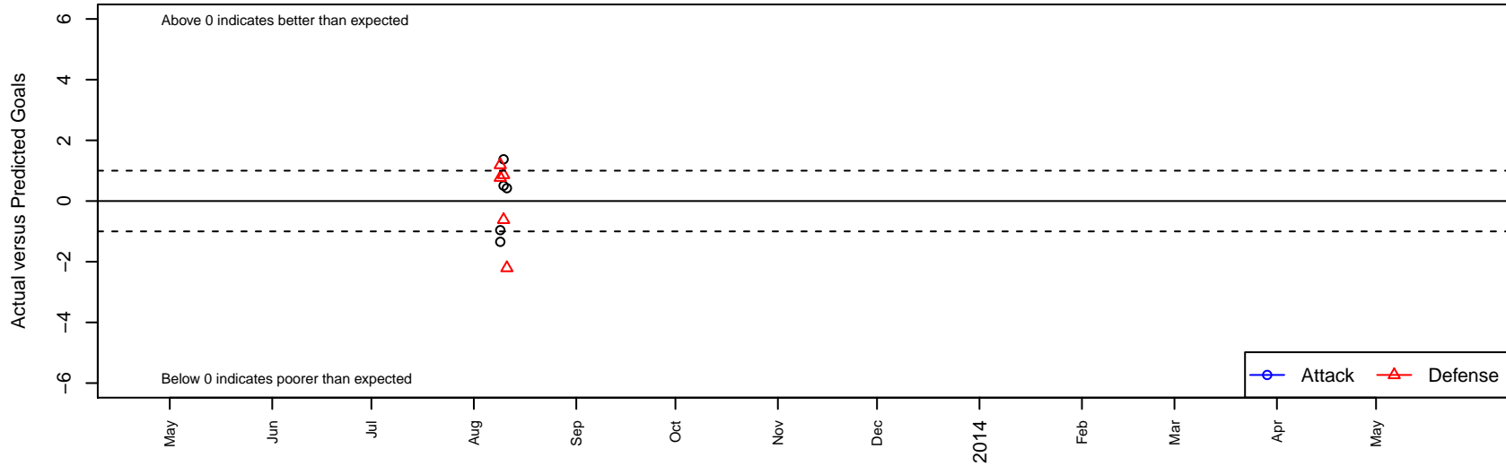
Barcelona Bay Area Academy G02 Dots are actual minus expected GF (blue circles) and GA (red triangles). Blue line is smoothed change in attack strength. Red is smoothed change in defense strength.
